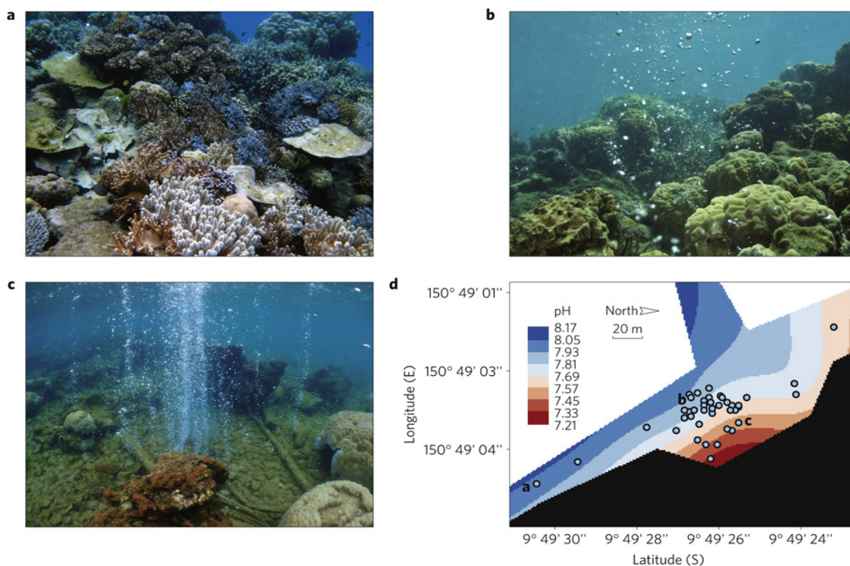
Figure 3. Seascapes at: a) control site (low \text{pCO}_2 : pH~8.1); b) moderate seeps (high \text{pCO}_2 : pH 7.8–8.0); and c) the most intense vents (pH<7.7), showing progressive loss of diversity and structural complexity with increasing \text{pCO}_2 . d) Map of the main seep site along the western shore of Upa-Upasina. Color contours indicate seawater pH, and the letters indicate the approximate locations of seascapes as shown in a–c. Nature Climate Change, (Fabricius et al. 2011).
