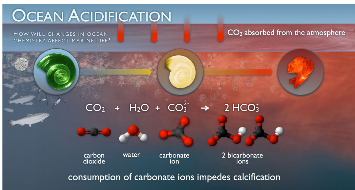
Figure 2. Schematic diagram of ocean acidification processes in the sea (image provided by the NOAA Pacific Marine Environmental Laboratory Carbon Group in collaboration with the University of Washington Center for Environmental Visualization).
