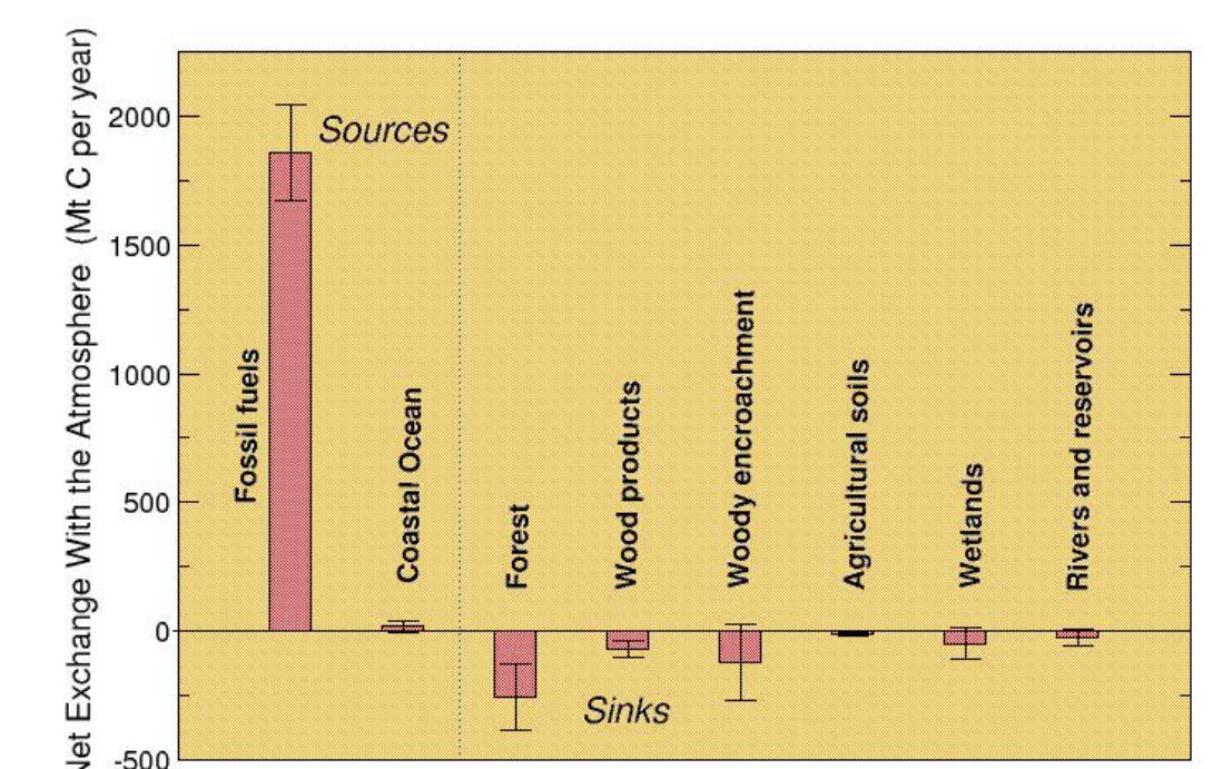
North American carbon sources and sinks (million tons carbon per year). Sources add carbon dioxide to the atmosphere (bars above the zero line); sinks remove it (bars below the zero line). Error bars indicate the uncertainty in that estimate. North America is currently a net carbon source (1330 ± 333 Mt C yr -1 ). 6
